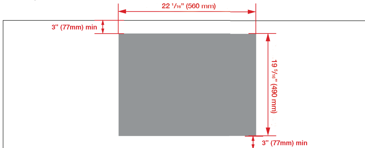
Countertop Cutout
