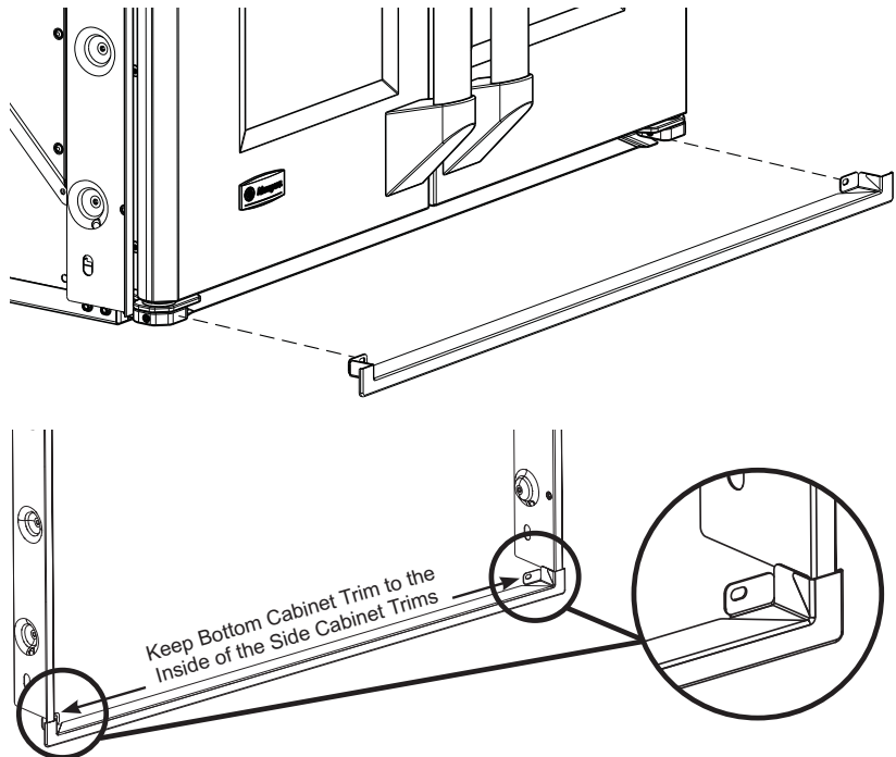
SWO's installation
