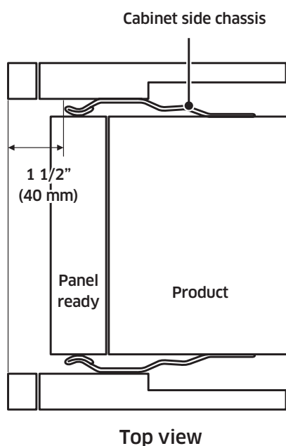
Overlay Type
