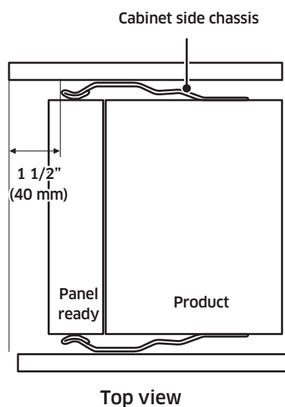
Frameless Type
